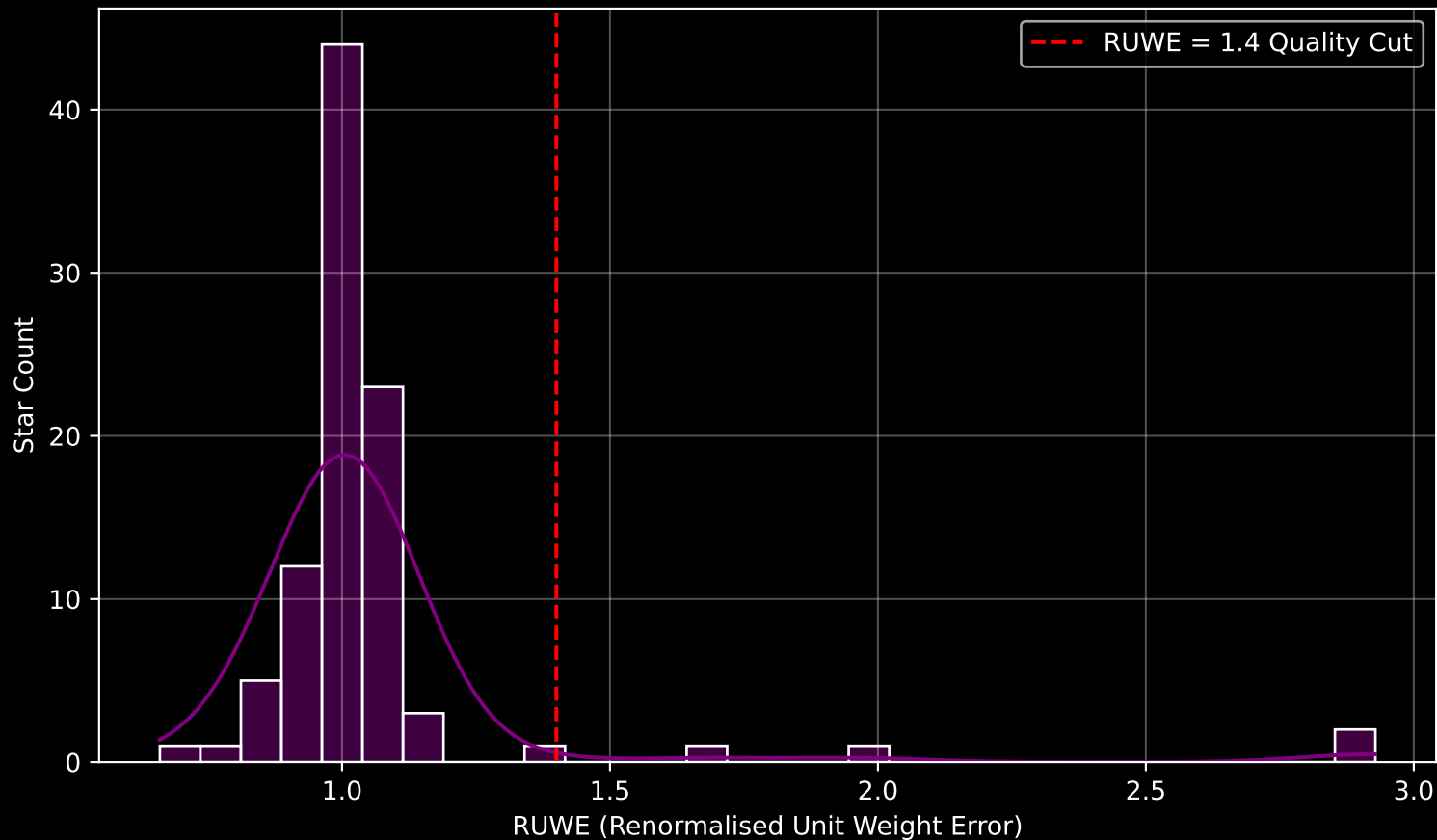
GAPOGEE DR17 Field [LMC13] RUWE Distribution (n= 94)
