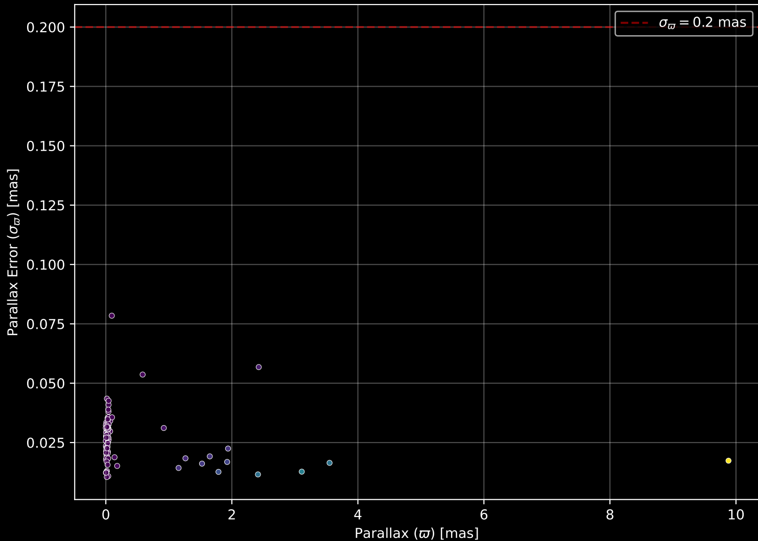
APOGEE DR17 Field: [LMC13] Parallax Quality (n= 94)
