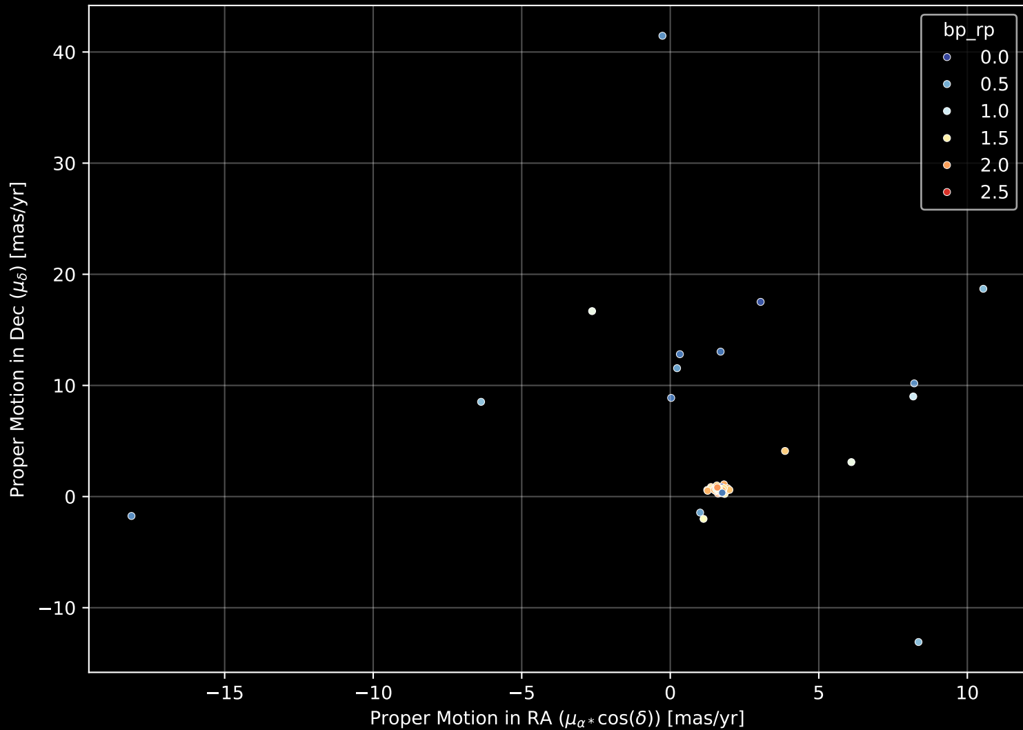
APOGEE DR17 Field: [LMC13] Proper Motion Diagram (n= 94)
