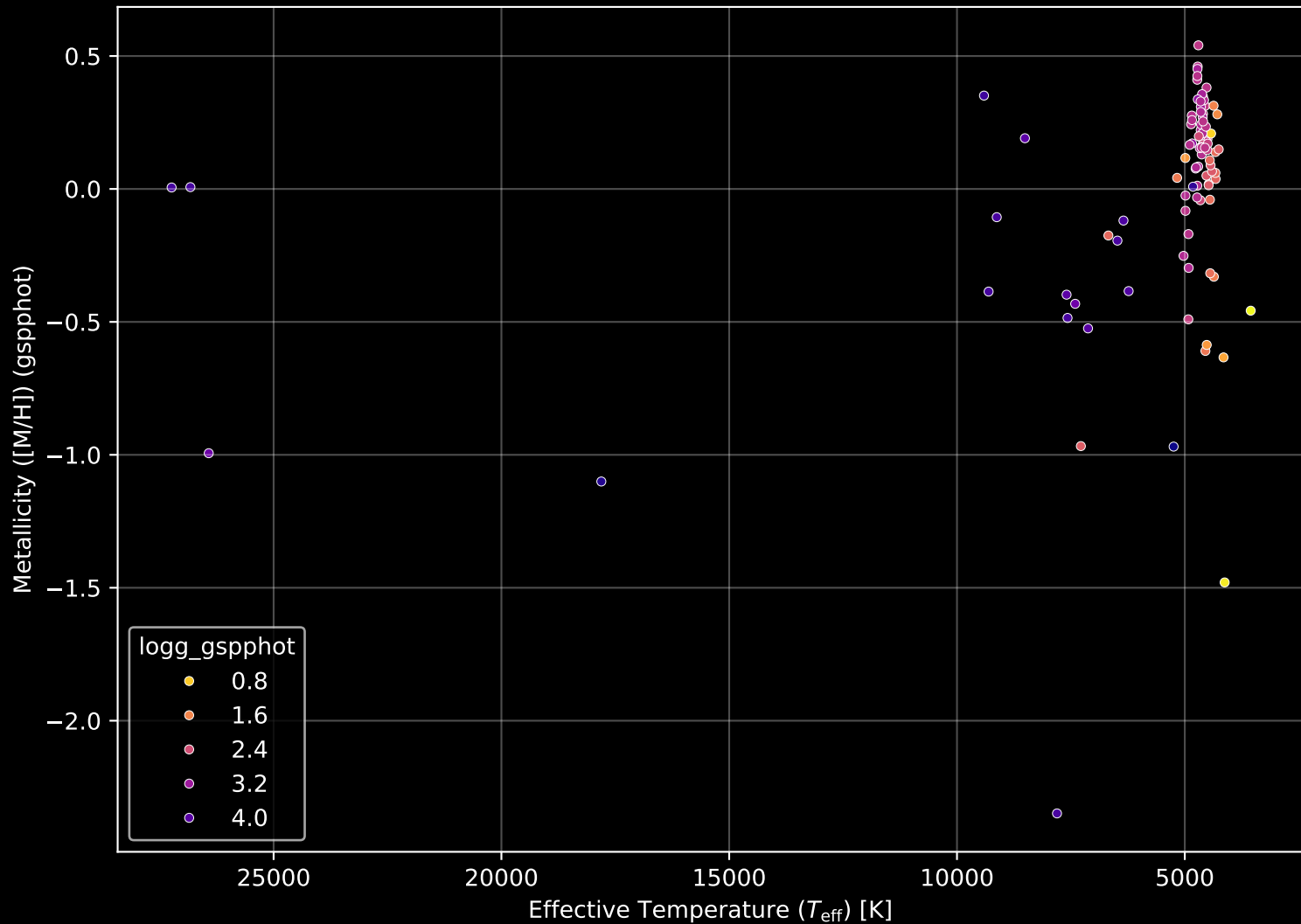
APOGEE DR17 Field: [LMC13] Stellar Population Parameters (n= 94)
