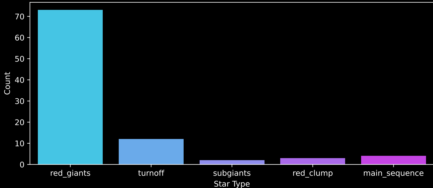
APOGEE DR17 Field: [LMC13] Count plot of Star Type
