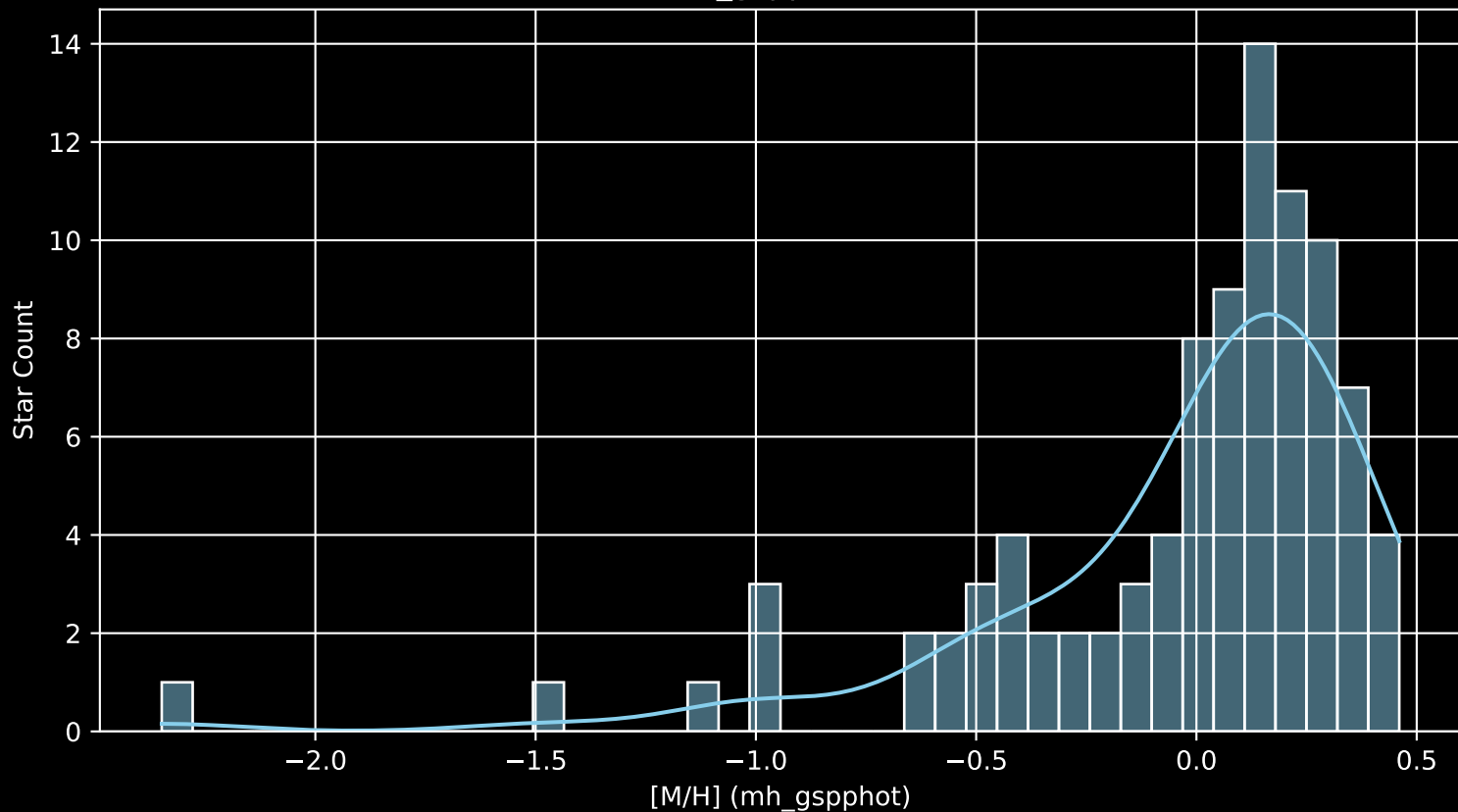
APOGEE DR17 Field: [LMC13 [M/H] (mh_gspphot) (n= 93)
